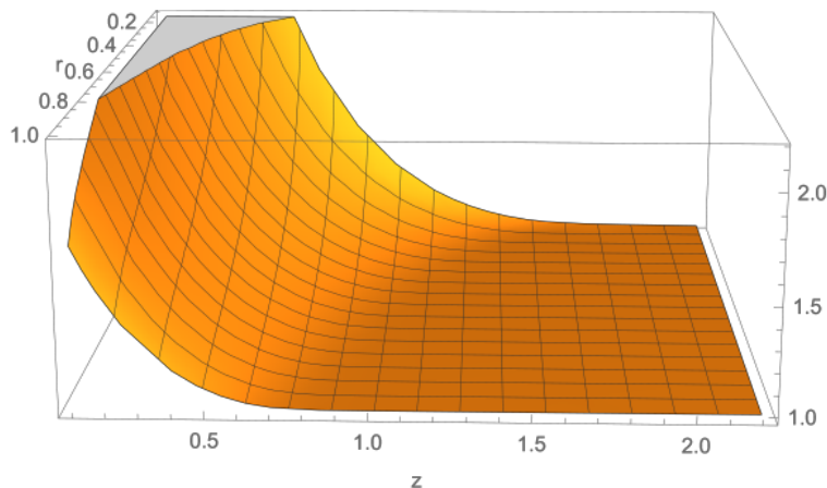
FIGURE 4. Plot of U in the case \rho(r) = \sqrt{r_0 + r} .
