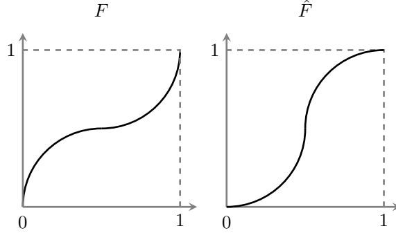
Figure 3: An example of a cumulative distribution function F and its conjugate \hat{F} . The shapes under the curves are congruent: the transformation that maps one to the other is reflection around the anti-diagonal. Qualitatively, F corresponds to the belief distribution of a more informative signal, and \hat{F} corresponds to that of a less informative signal.
