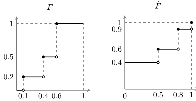
Figure 5: The conjugate of a discrete distribution F with three atoms at 0.1, 0.4, and 0.6. Each atom becomes an interval of zero measure with length equal to the atom's weight, and vice versa. Since F does not have atoms at the endpoints of [0, 1] , the number of intervals of zero measure exceeds the number of atoms by one, so its conjugate \hat{F} has four atoms at 0, 0.5, 0.8, and 1.
