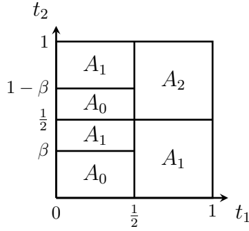
Figure 8: In the private private information structure associated with the partition (A_0, A_1, A_2) , the signal t_1 induces the same distribution of posteriors as s_1 . For any parameter \beta \in [0, 1/2] , this partition is a partition of uniqueness and, hence, we get a one-parametric family of non-equivalent optimal disclosures given by the signal t_2 .
