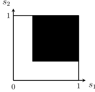
Figure 7: A social welfare maximizing private information structure for the decision problem in which u_1(\omega, a) = u_2(\omega, a) = 2|\omega - a| - 1 .
